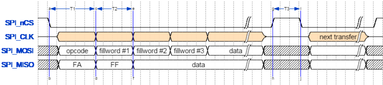
Figure 9: SPI timing
