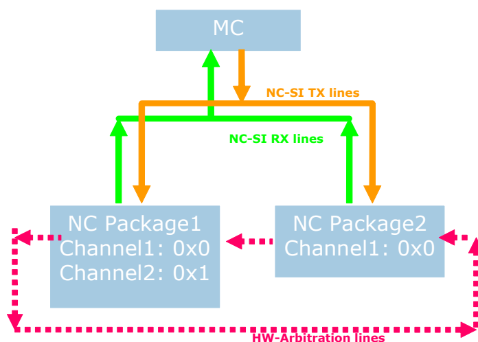
Figure 10-10 Multi-NC Environment
