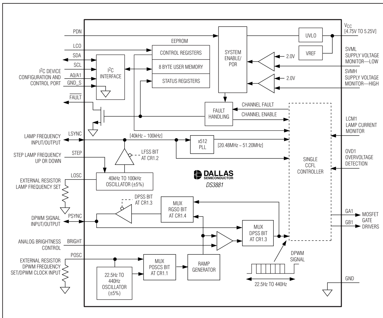
Figure 1. Functional Diagram
