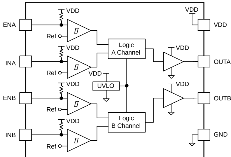
Figure 1. NCP81071 Dual Non-inverting Block Diagram
