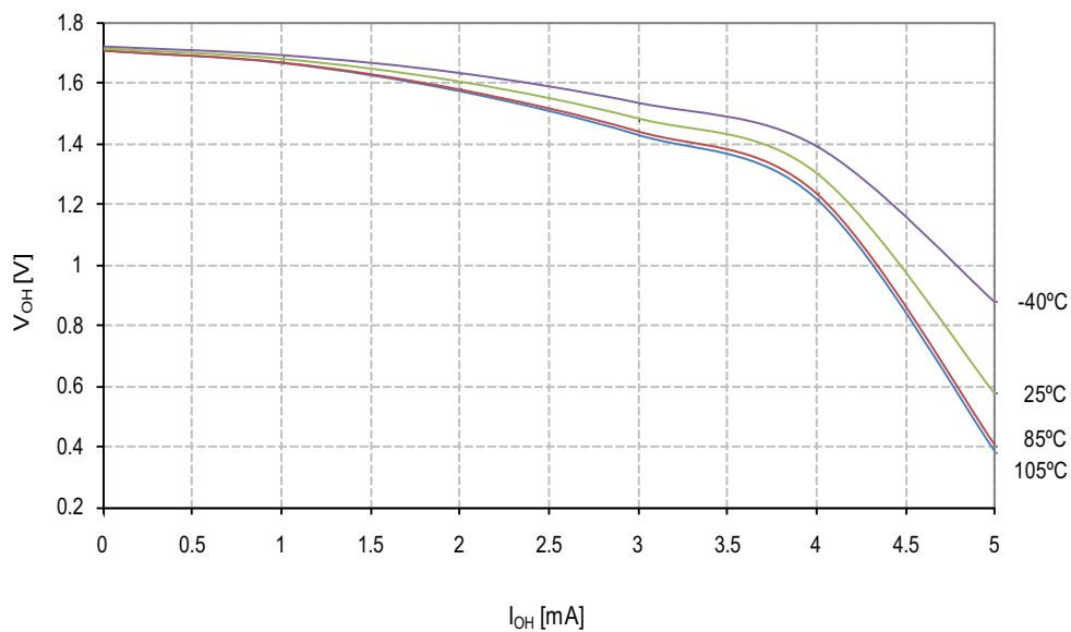
Figure 26-34. V_{OH} : Output Voltage vs. Source Current (I/O Pin, V_{CC} = 1.8V )
