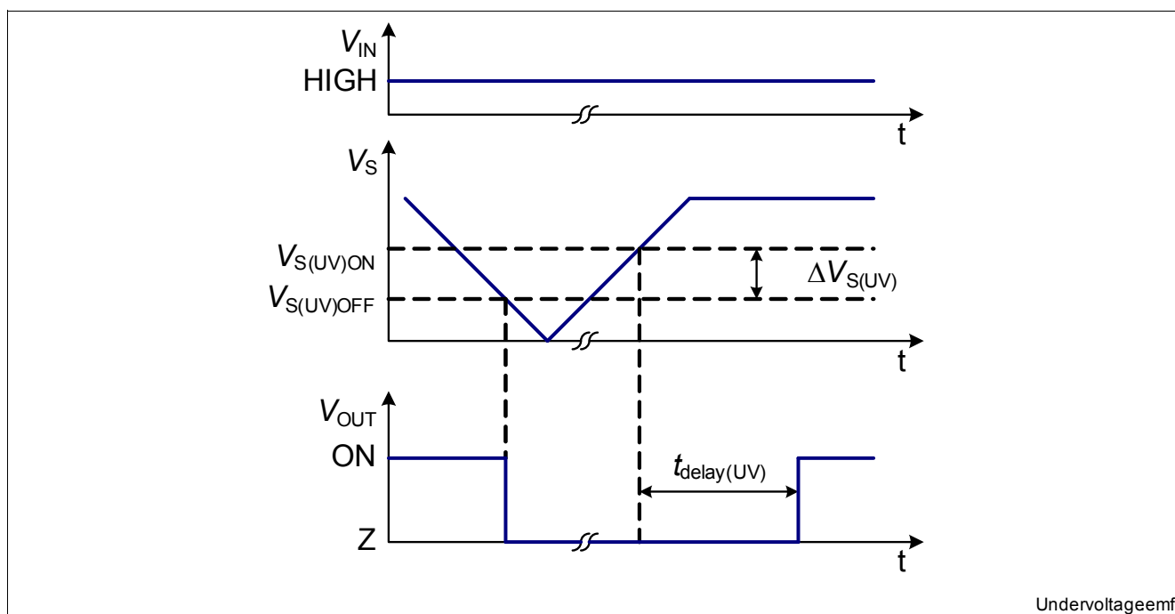
Figure 24 Undervoltage shutdown and restart
