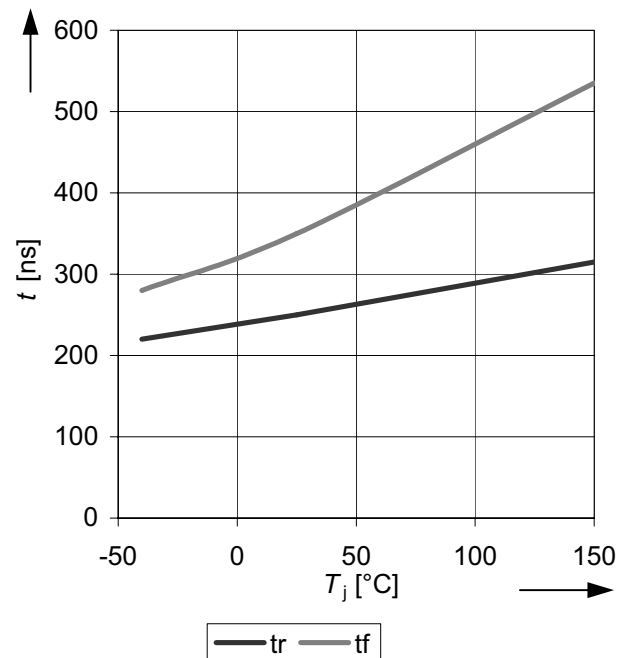
Figure 32 Typical turn ON rise time t_r and turn OFF fall time t_f as a function of the junction temperature T_j R_L = 1\Omega , V_S = 13.5V , 10\% \leq 90\% V_S
