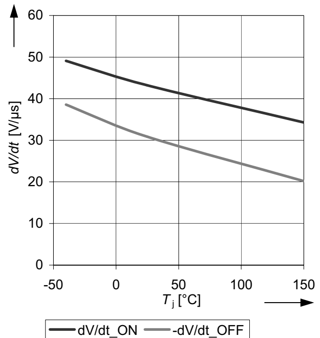
Figure 30 Typical slew rate for turn ON (dV/dt)_{ON} and turn OFF -(dV/dt)_{OFF} as a function of the junction temperature T_j R_L = 1\Omega , V_S = 13.5V , 30\% \leq 70\% V_S
