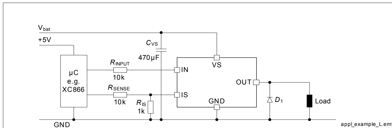
Figure 45 Application Diagram for switching an inductive load without external circuitry supporting open load detection in OFF state
