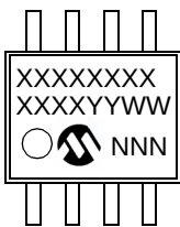
8-Lead Plastic Small Outline (SOIC)
