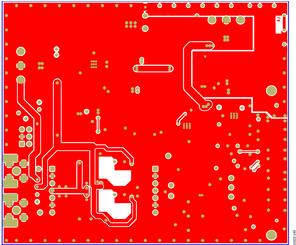
Figure 40. 10-Lead Evaluation Board, Layer 4
