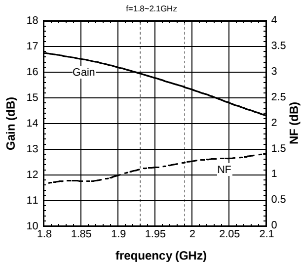
Gain, NF vs. frequency
