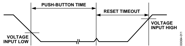
Figure 12. Push-Button Reset Timing Diagram
