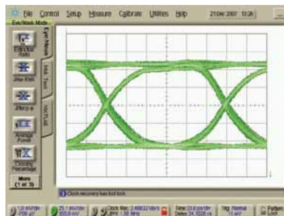
Eye Diagram
