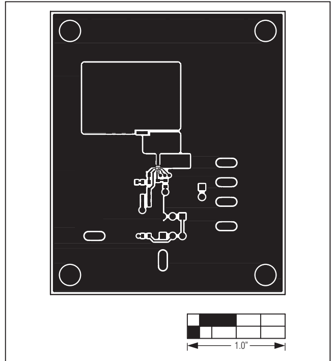
Figure 3. MAX15058 EV Kit Component PCB Layout—Component Side
