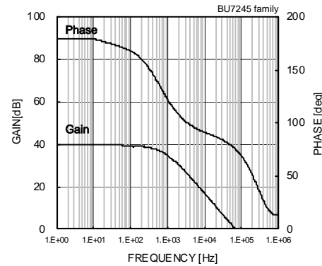
Fig.92 Gain – Frequency
