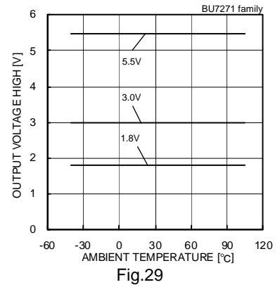
Output Voltage High - Ambient Temperature (RL=10[kΩ])
