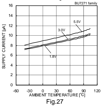
Supply Current - Ambient Temperature
