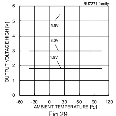
Output Voltage High - Ambient Temperature (RL=10[kΩ])
