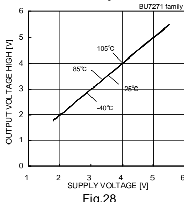
Output Voltage High - Supply Voltage (RL=10[kΩ])
