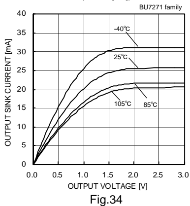
Output Sink Current – Output Voltage (VDD=3[V])
