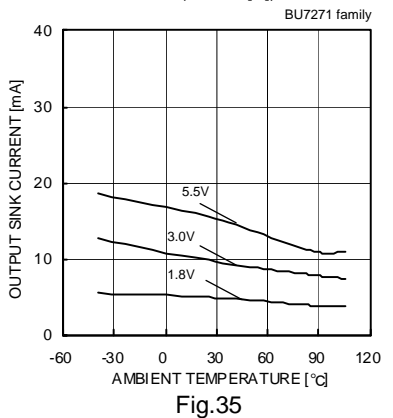
Output Sink Current – Ambient Temperature (VOUT=VSS+0.4[V])
