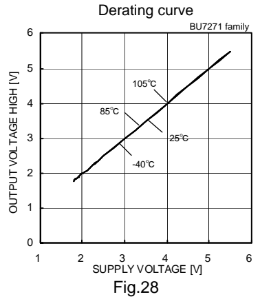
Output Voltage High – Supply Voltage (RL=10[kΩ])
