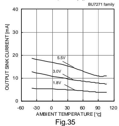
Output Sink Current – Ambient Temperature (VOUT=VSS+0.4[V])
