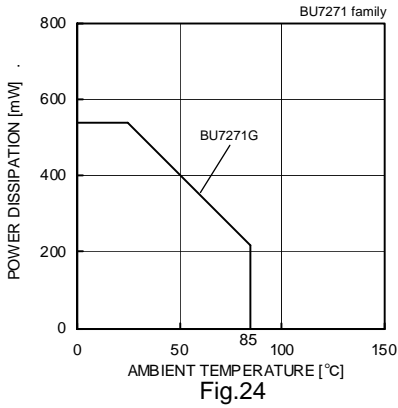
Derating curve
