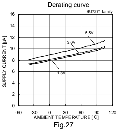
Supply Current – Ambient Temperature
