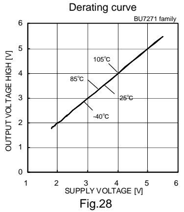
Output Voltage High – Supply Voltage (RL=10[kΩ])
