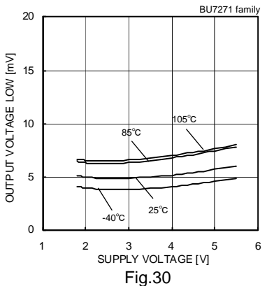
Output Voltage Low – Supply Voltage (RL=10[kΩ])
