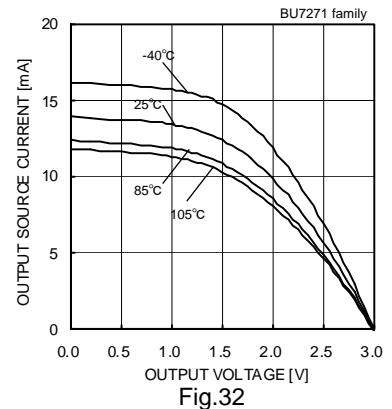
Output Source Current – Output Voltage (VDD=3[V])
