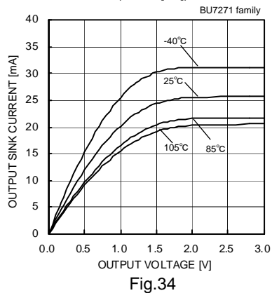
Output Sink Current – Output Voltage (VDD=3[V])
