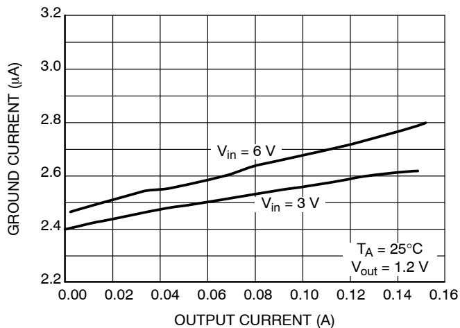
Figure 4. Ground Pin Current vs. Output Current
