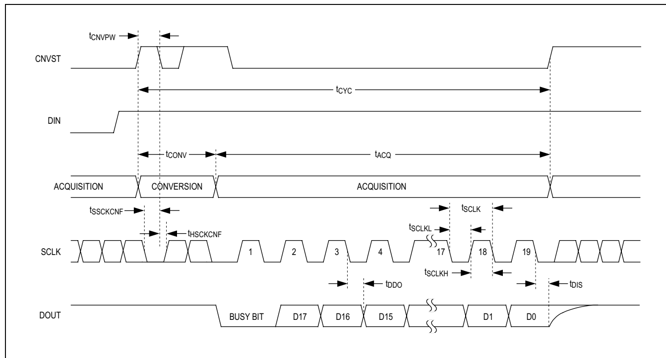
Figure 9. CS With Busy Indicator Mode Timing
