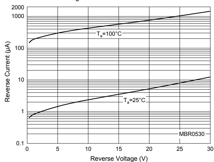
Fig. 2 - Reverse Characteristics
