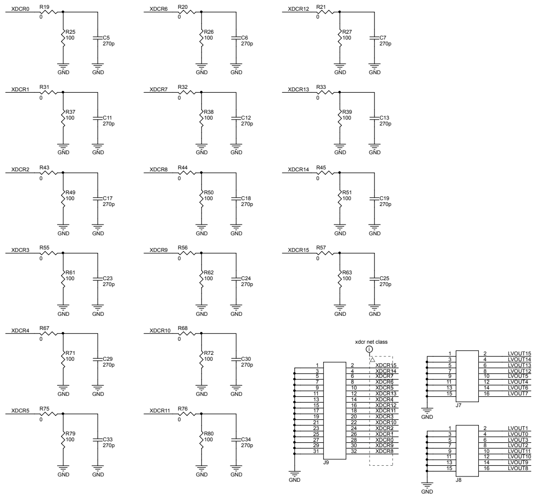
Figure 3. STEVAL-IME014V1 schematic 3
