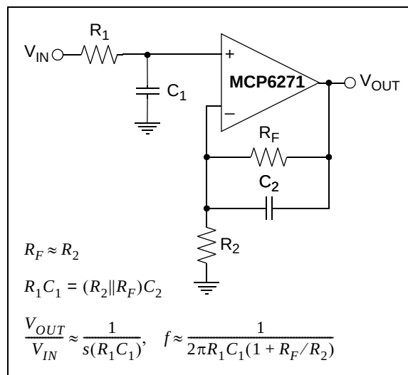
FIGURE 4-9: Non-Inverting Integrator.
