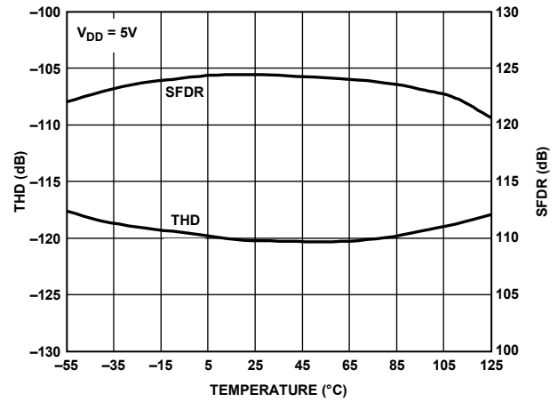
Figure 16. THD, SFDR vs. Temperature
