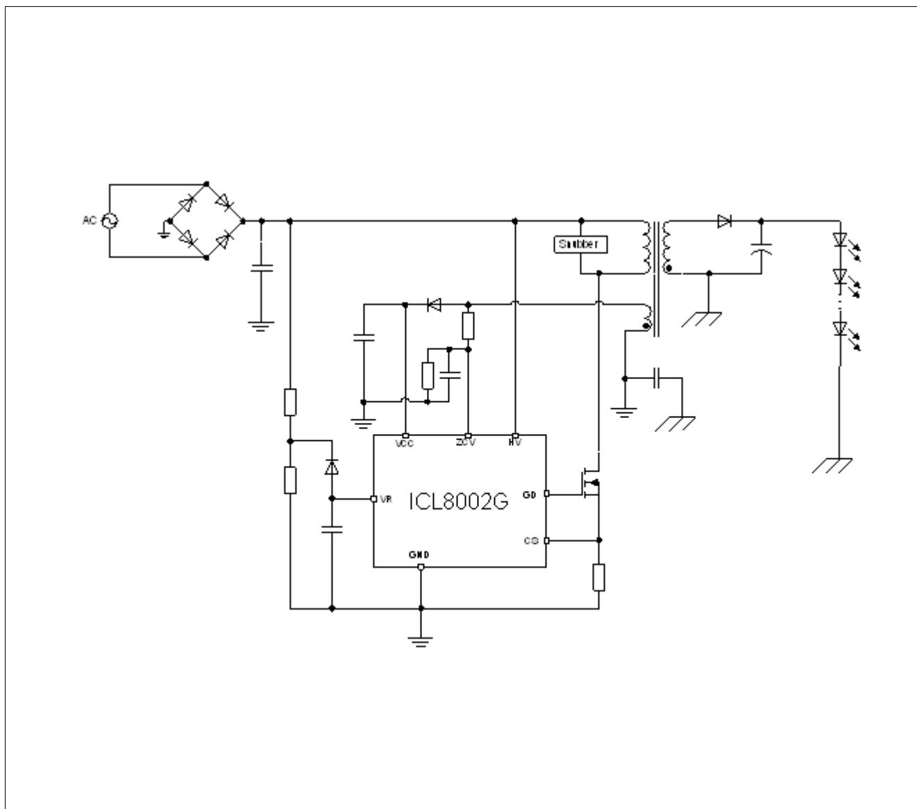
Figure 1 Application Circuit
