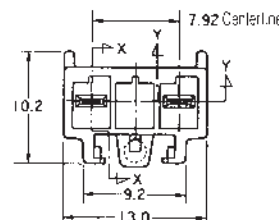
Section Y-Y
