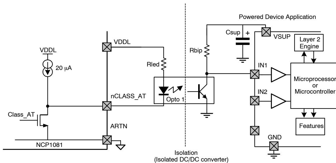
Figure 8. Isolated nClass AT Communication with the Powered Device Application
