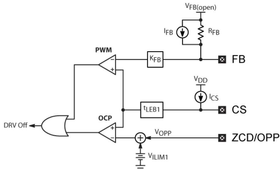
Figure 8. OPP Circuit Schematic
