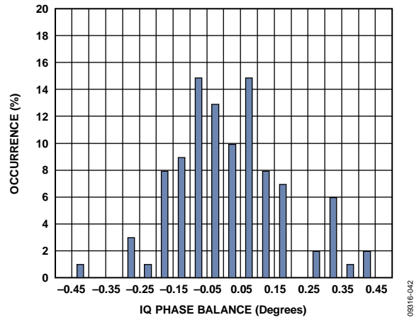
Figure 45. IQ Phase Balance, Narrow-Band Mode, Nominal Conditions
