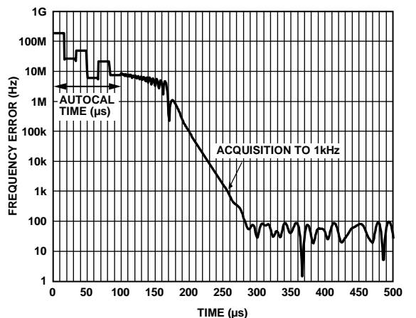
Figure 58. PLL Acquisition
