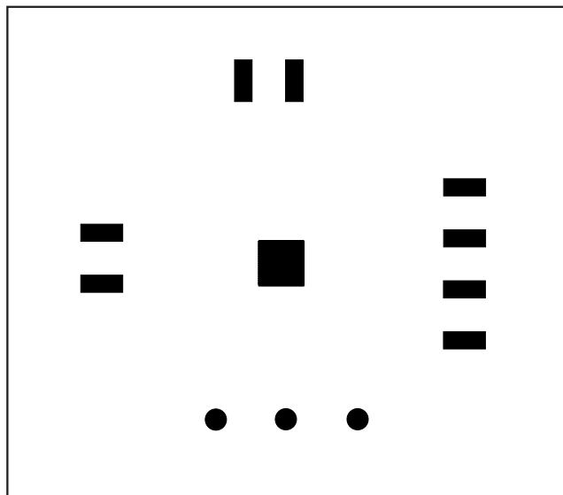
Figure 9. MAX9994 EV Kit PC Board Layout—Bottom Soldermask
