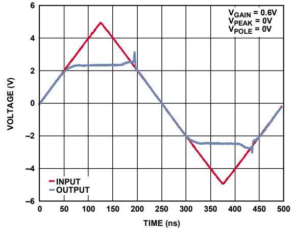
Figure 10. Overdrive Recovery
