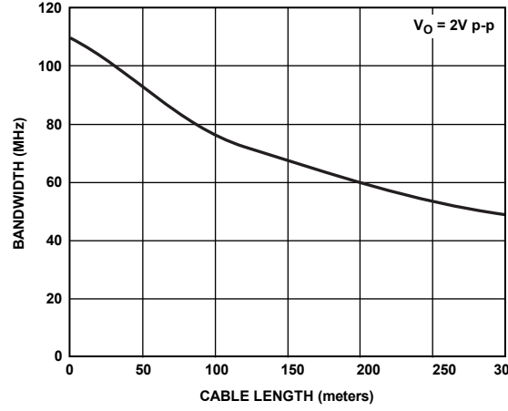
Figure 9. Equalized -3 dB Bandwidth vs. Cable Length
