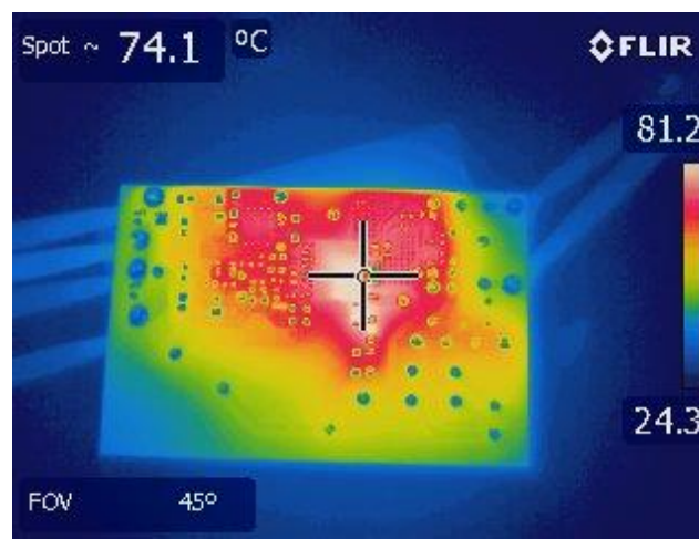
Figure 21 – InnoSwitch-EP Side. 85 VAC, Full Load.
