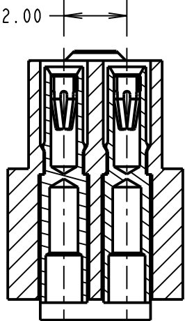
SECTION X-X
