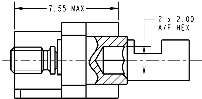
PART SECTION Y-Y
