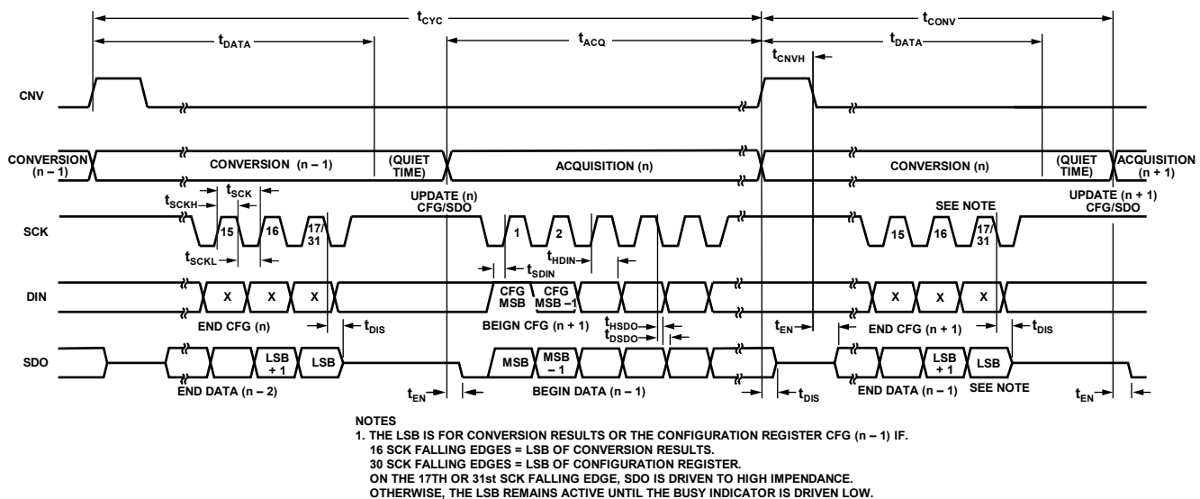
Figure 40. Serial Interface Timing for the AD7699 with a Busy Indicator
