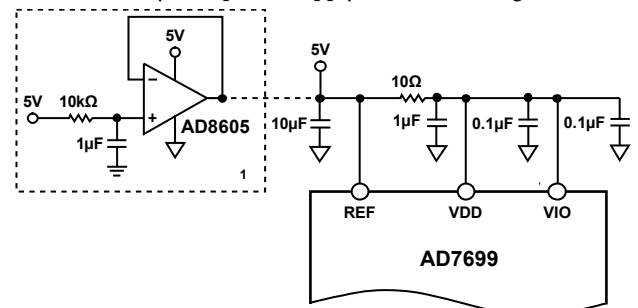
Figure 34. Example of an Application Circuit
