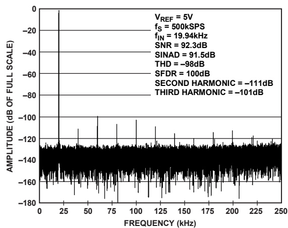
Figure 7. 20 kHz FFT, VREF = 5 V
