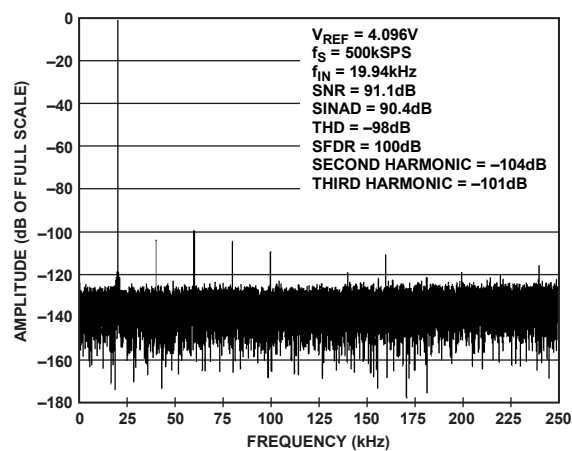
Figure 10. 20 kHz FFT, VREF = 4.096 V
