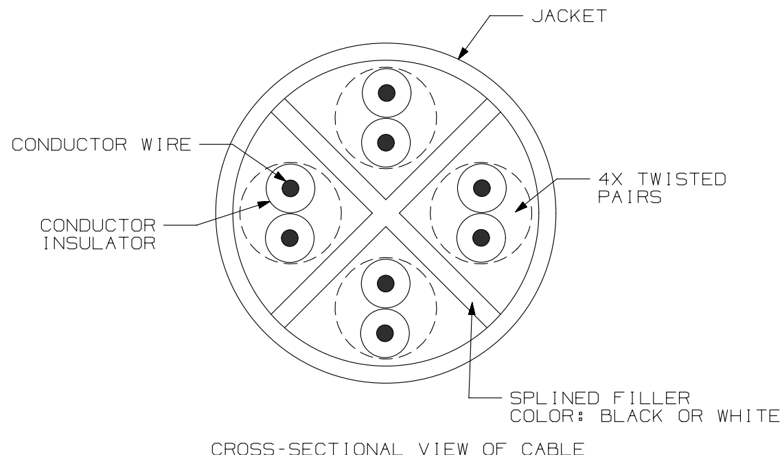
CROSS-SECTIONAL VIEW OF CABLE
