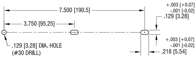
SUGGESTED MOUNTING DETAIL
