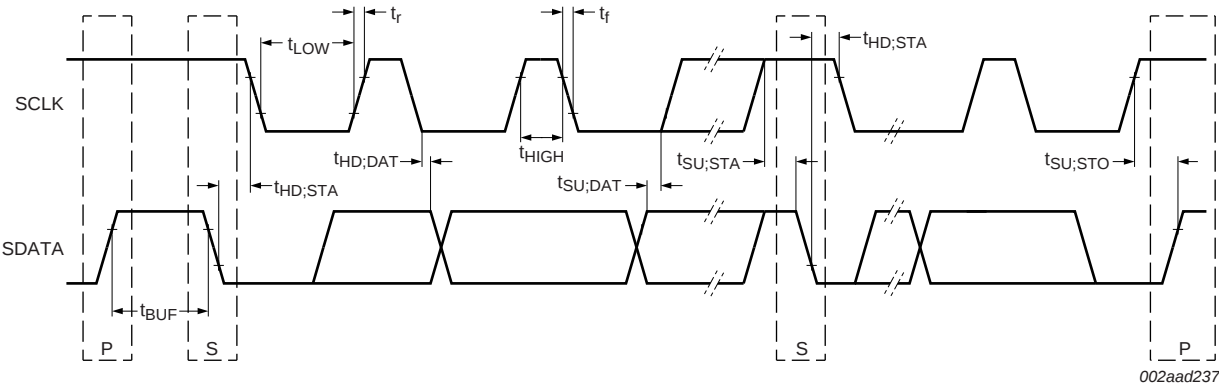
Fig 12. Timing measurements
