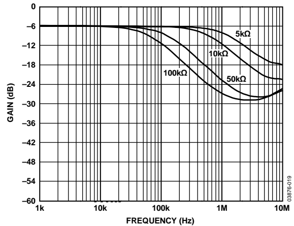
Figure 21. -3\text{ dB} Bandwidth @ Code = 0x80
