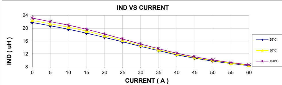
HA55L-3023135LF*
