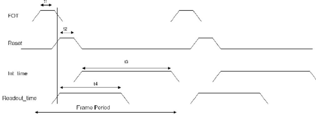
Figure 23. Timing Diagram
