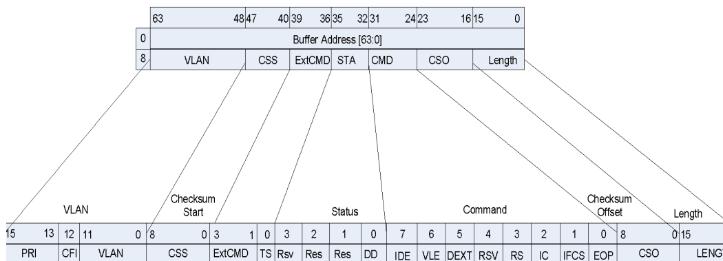
Figure 34. Legacy Transmit Descriptor Format
