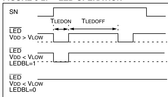
FIGURE 5-2: LED OPERATION
