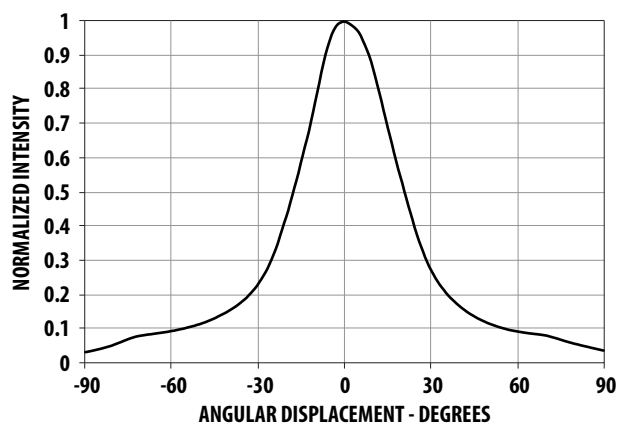
Figure 8. Radiation pattern for AMBER - Minor Axis
