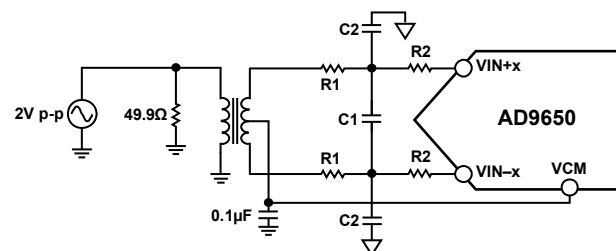
Figure 80. Differential Transformer-Coupled Configuration
