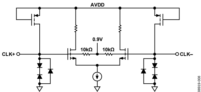
Figure 69. Equivalent Clock Input Circuit
