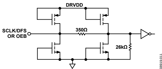
Figure 72. Equivalent SCLK/DFS or OEB Input Circuit
