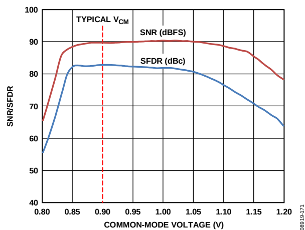
Figure 67. SNR/SFDR vs. Input Common Mode (VCM) with f_{IN} = 30.3 \text{ MHz}
