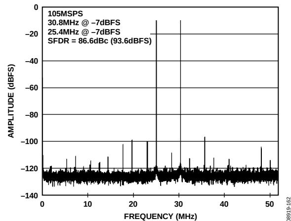
Figure 59. AD9650-105 Two-Tone FFT with f_{IN1} = 25.4 MHz and f_{IN2} = 30.8 MHz
