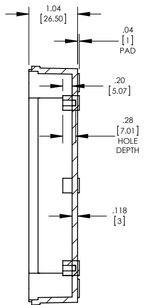
SECTION E-E
