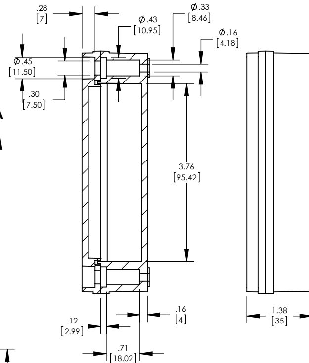
SECTION C-C
